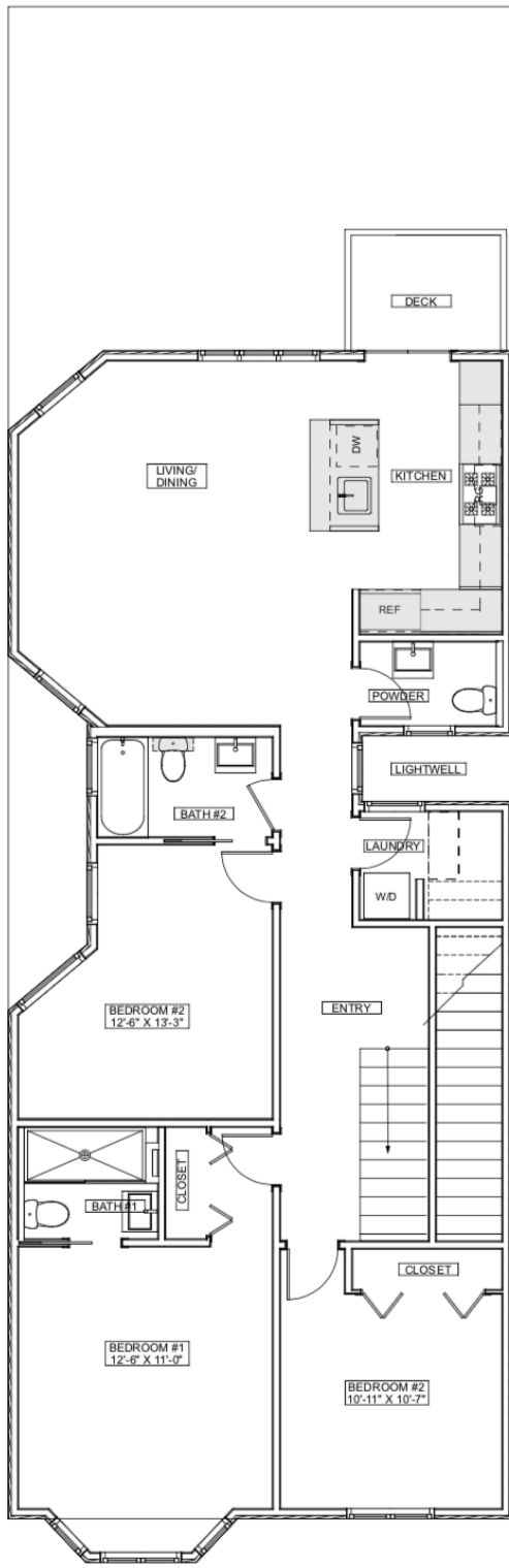
2ND FLOOR
